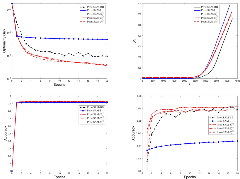
Fig. 4: Test problem NN- L_1 for the IJCNN dataset - First row: averaged optimality gap computed on the training set (left panel) and increase of the average of the mini-batch size (right panel). Second row: averaged accuracy evaluated on the test set (left panel) and a zoom of the accuracy in the interval [0.90, 0.93] (right panel).
