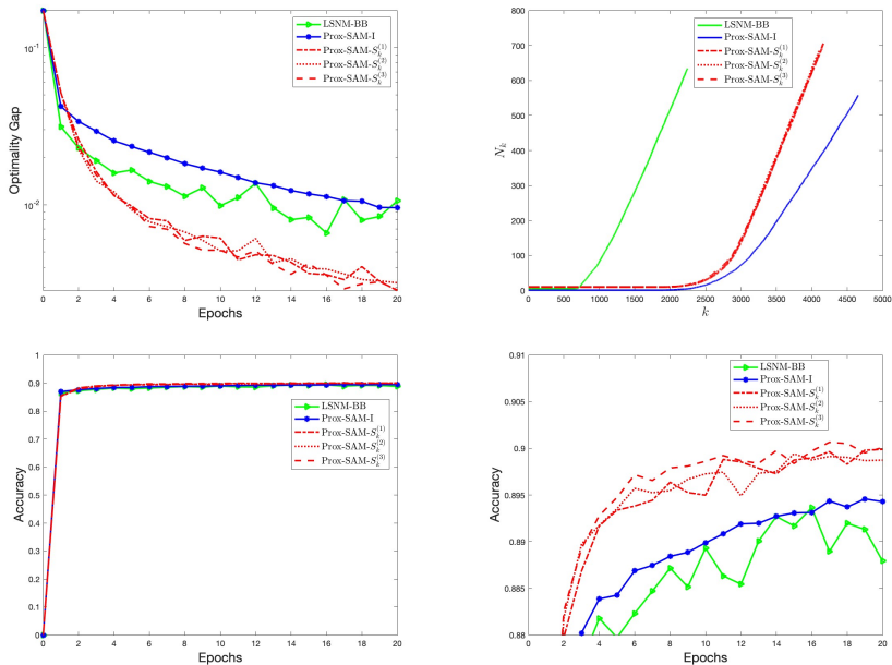
Fig. 8: Test problem NN-L_2 for the MNIST dataset - First row: averaged optimality gap computed on the training set (left panel) and increase of the averaged mini-batch size (right panel). Second row: averaged accuracy evaluated on the test set (left panel) and a zoom of the accuracy in the interval [0.88, 0.91] (right panel).
