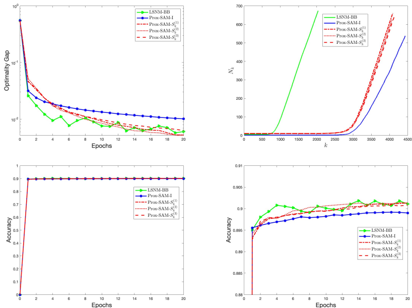
Fig. 7: LR- L_2 test problem for the w8a dataset - First row: averaged optimality gap computed on the training set (left panel) and increase of the averaged mini-batch size (right panel). Second row: averaged accuracy evaluated on the test set (left panel) and a zoom of the accuracy in the interval [0.88, 0.91] (right panel).
