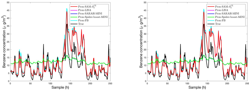
Fig. 13: Estimated benzene concentrations during 10 days (240 hours) obtained by solving the nonlinear regression problem with L_1 regularized problem (left panel) and the L_2 regularized problem (right panel) using the compared methods; the black line represents the true concentration.
