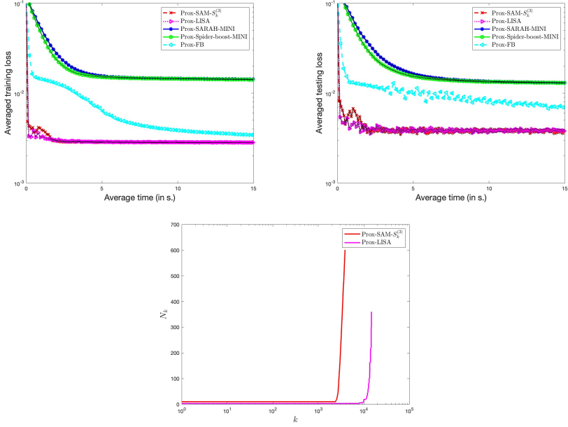
Fig. 12: Results for the nonlinear regression with L_2 regularization term - First row: averaged loss computed over the training set (left panel) and averaged loss computed over the testing set (right panel). Second row: increase of the averaged mini-batch size.
