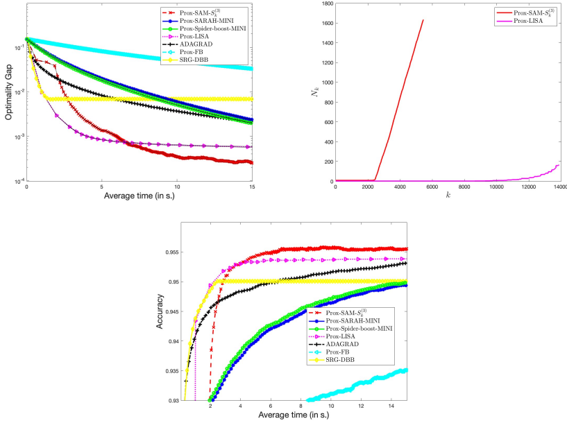
Fig. 10: Behavior of the methods in a time budget of 15 seconds for the test problem \text{NN-}L_2 and the \text{RCV1} dataset - First row: averaged optimality gap computed on the training set (left panel) and increase of the averaged mini-batch size (right panel). Second row: averaged accuracy evaluated on the test set.
