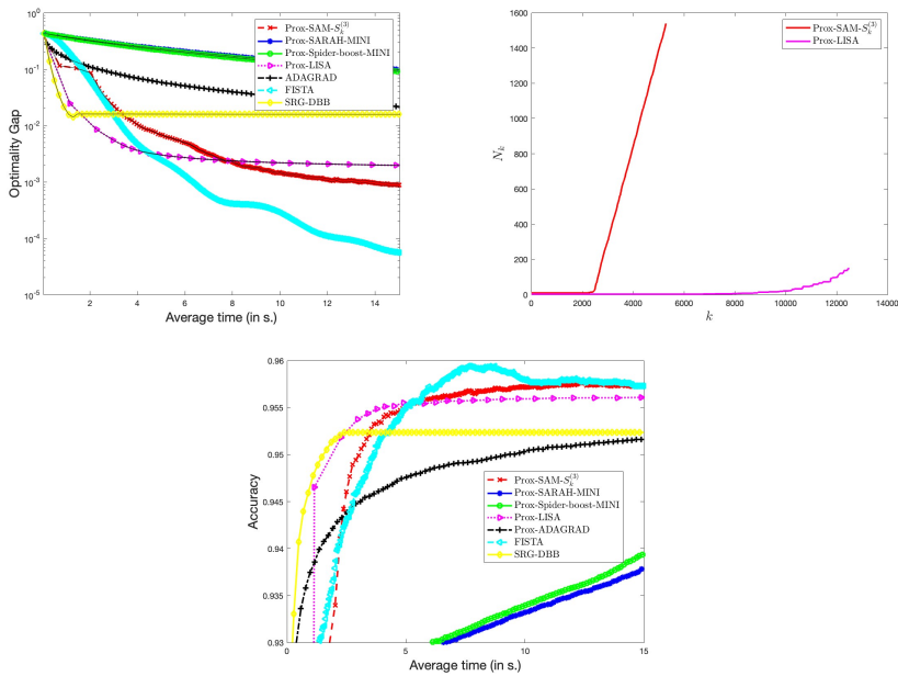
Fig. 9: Behavior of the methods in a time budget of 15 seconds for the test problem LR- L_2 and the RCV1 dataset - First row: averaged optimality gap computed on the training set (left panel) and increase of the averaged mini-batch size (right panel). Second row: averaged accuracy evaluated on the test set.
