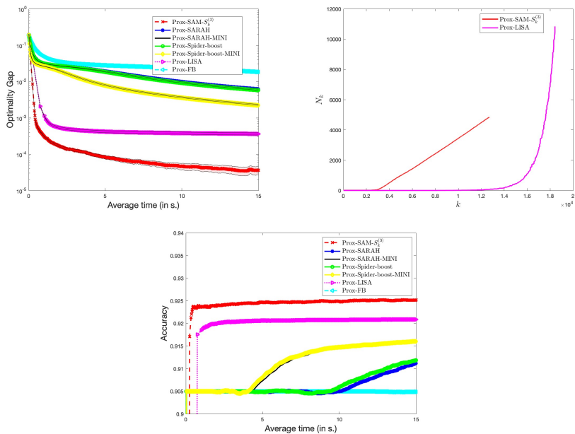
Fig. 6: Behavior of the methods in a time budget of 15 seconds for the test problem NN-L_1 and the IJCNN dataset - First row: averaged optimality gap computed on the training set (left panel) and increase of the averaged mini-batch size (right panel). Second row: averaged accuracy evaluated on the test set.
