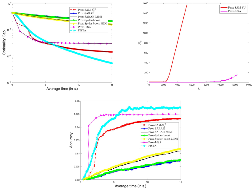
Fig. 5: Behavior of the methods in a time budget of 15 seconds for the test problem LR-L_1 and the RCV1 dataset - First row: averaged optimality gap computed on the training set (left panel) and increase of the averaged mini-batch size (right panel). Second row: averaged accuracy evaluated on the test set.
