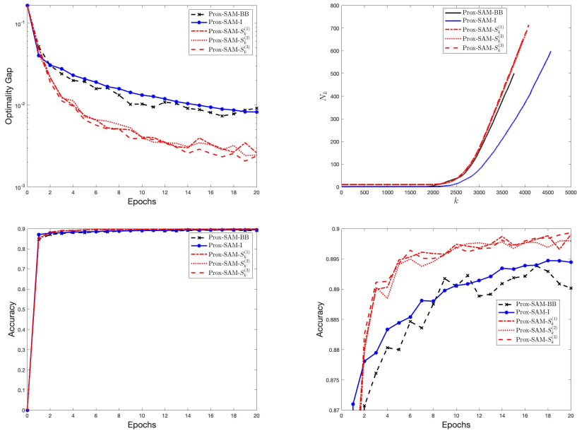
Fig. 2: Test problem NN-L_1 for the MNIST dataset - First row: averaged optimality gap computed on the training set (left panel) and increase of the average of the mini-batch size (right panel). Second row: averaged accuracy evaluated on the test set (left panel) and a zoom of the accuracy in the interval [0.87, 0.90] (right panel).
