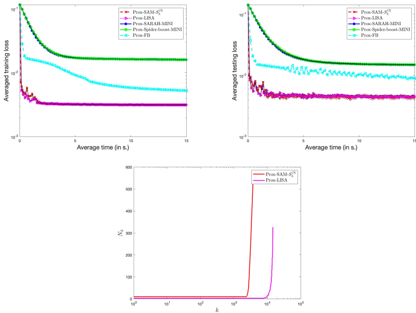
Fig. 11: Results for the nonlinear regression with L_1 regularization term - First row: averaged loss computed over the training set (left panel) and averaged loss computed over the testing set (right panel). Second row: increase of the averaged mini-batch size.
