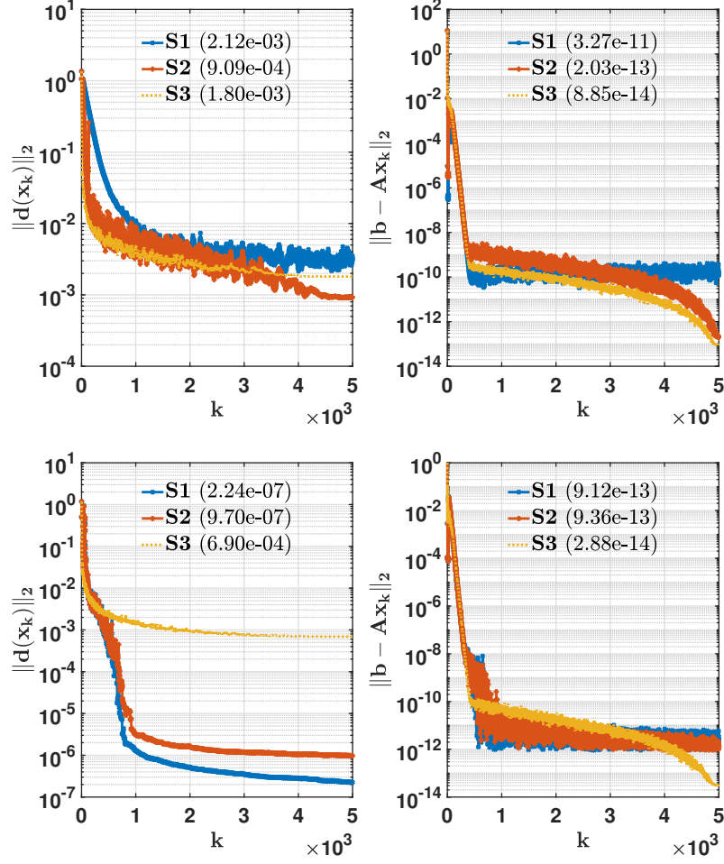
Fig. 2: The average values of \|d(x_k)\| and \|Ax_k - b\| over ten runs using strategies S1–S3 on MNIST (top) and MUSHROOMS (bottom)
