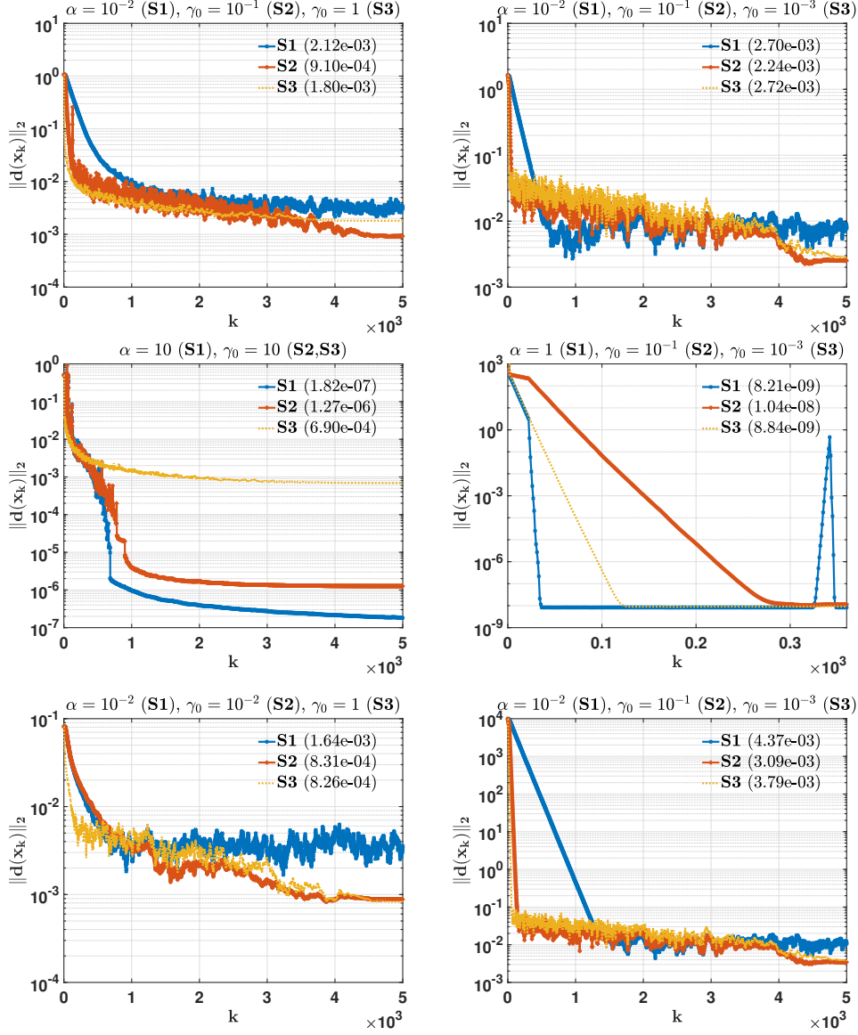
Fig. 1: The average values of \|d(x_k)\| over ten runs using strategies S1–S3 ; left column: MNIST (top), MUSHROOMS (middle), DIABETES (bottom), and right column: DT0C1L (top), HUESTIS (middle), and Hs50 (bottom)
