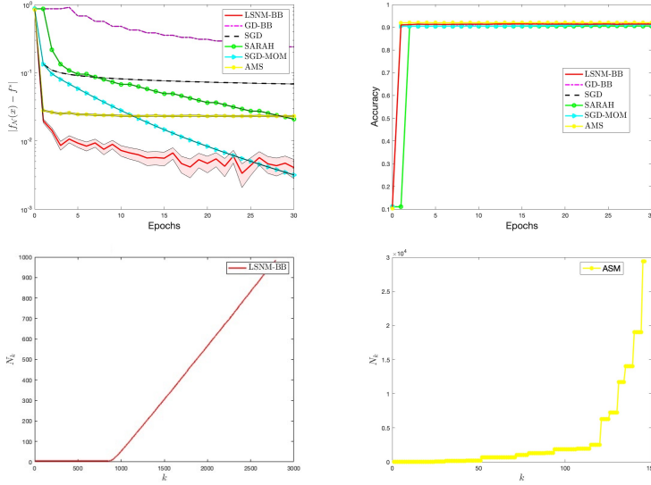
Fig. 7: Dataset IJCNN and objective function with LR loss terms - First row: on the left, behaviour of the averaged optimality gap (combined with the relative standard deviation) computed at the training set with respect to the epochs; on the right, averaged accuracy evaluated at the testing set with respect to the epochs. Second row: increase of the averaged mini-batch size with respect to the iterations for LSNM-BB method (on the left) and for ASM method (on the right).
