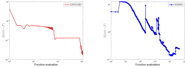
Fig. 9: Dataset w8a and objective function with LR loss terms - Behaviour of the optimality gap computed at the training set with respect to the function evaluations in the first epoch for LSNM-BB on the left and for SLiSeS on the right. A logarithmic scale is used for both axes.
