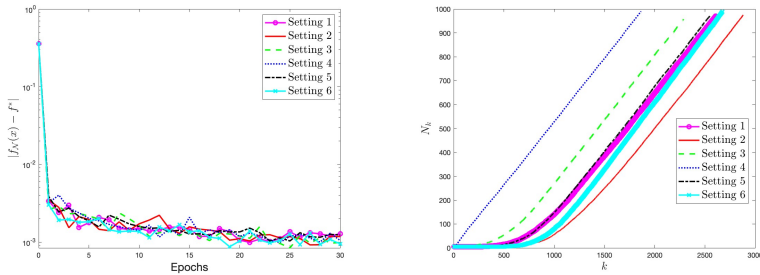
Fig. 6: Results obtained by LSNM-BB Algorithm for the dataset IJCNN and the objective function with NN loss terms - On the left, behaviour of the averaged optimality gap computed at the training set with respect to the epochs for the six starting settings of c_{min} , C_{max} and \zeta_k . On the right, increase of the averaged mini-batch size with respect to the iterations for LSNM-BB Algorithm equipped with the six starting settings of c_{min} , C_{max} and \zeta_k .
