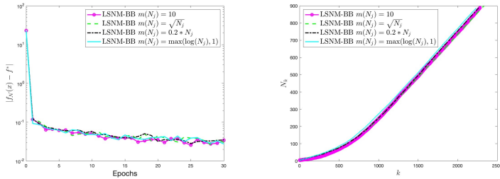
Fig. 1: Results obtained by LSNM-BB Algorithm for the dataset MNIST and objective function with LR loss terms - On the left, behaviour of the averaged optimality gap with respect to the epochs in the case of the four rules for m(N_j) ; on the right, corresponding behaviour of the averaged mini-batch size with respect to the iterations.
