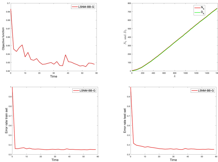
Fig. 15: Behavior of LSNM-BB-G Algorithm. First row: on the left panel, objective function evaluated for the training set every two seconds; on the right panel, the increase of the mini-batch sizes N_k and D_k . Second row: on the left panels, error rate computed at the training set every two seconds; on the right panel, error rate computed at the testing set every two seconds.
