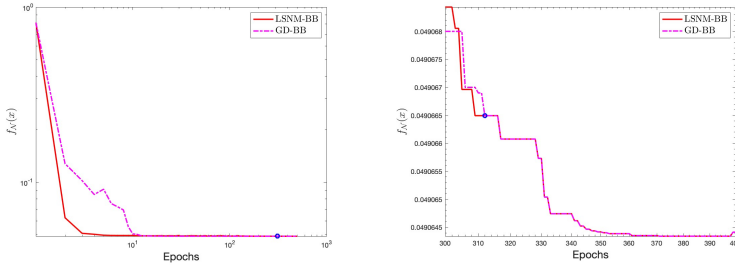
Fig. 14: Dataset w8a and objective function with NN loss terms - On the left, behaviour of the objective function for LSNM-BB and GD-BB methods along 500 epochs; on the right a zoom along 300 – 400 epochs is shown; at the epoch 312, LSNM-BB uses the whole dataset and the two methods exhibit the same behaviour.
