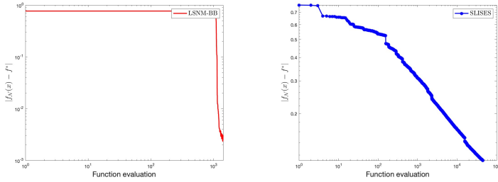
Fig. 10: Dataset w8a and objective function with NN loss terms - Behaviour of the optimality gap computed at the training set with respect to the function evaluations in the first epoch for LSNM-BB on the left and for SLiSeS on the right. A logarithmic scale is used for both axes.
