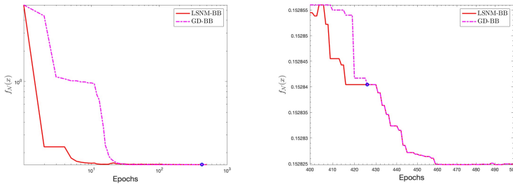
Fig. 13: Dataset w8a and objective function with LR loss terms - On the left, behaviour of the objective function for LSNM-BB and GD-BB methods along 500 epochs; on the right a zoom along 400 – 500 epochs is shown; at the epoch 426, LSNM-BB uses the whole dataset and the two methods exhibit the same behaviour.
