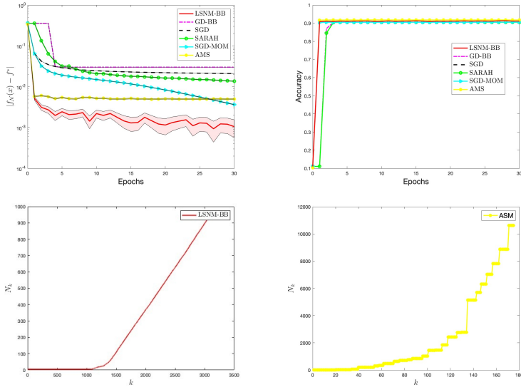
Fig. 8: Dataset IJCNN and objective function with NN loss terms - First row: on the left, behaviour of the averaged optimality gap (combined with the relative standard deviation) computed at the training set with respect to the epochs; on the right, averaged accuracy evaluated at the testing set with respect to the epochs. Second row: increase of the averaged mini-batch size with respect to the iterations for LSNM-BB method (on the left) and for ASM method (on the right).
