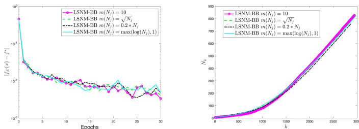
Fig. 3: Results obtained by LSNM-BB Algorithm for the dataset MNIST and objective function with NN loss terms - On the left, behaviour of the averaged optimality gap with respect to the epochs in the case of the four rules for m(N_j) ; on the right, corresponding behaviour of the averaged mini-batch size with respect to the iterations.
