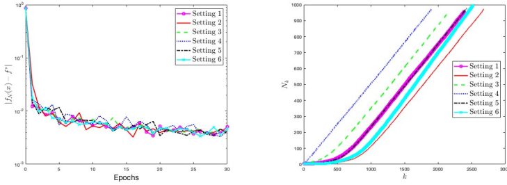
Fig. 5: Results obtained by LSNM-BB Algorithm for the dataset IJCNN and the objective function with LR loss terms - On the left, behaviour of the averaged optimality gap computed at the training set with respect to the epochs for the six starting settings of c_{min} , C_{max} and \zeta_k . On the right, increase of the averaged mini-batch size with respect to the iterations for LSNM-BB Algorithm equipped with the six starting settings of c_{min} , C_{max} and \zeta_k .
